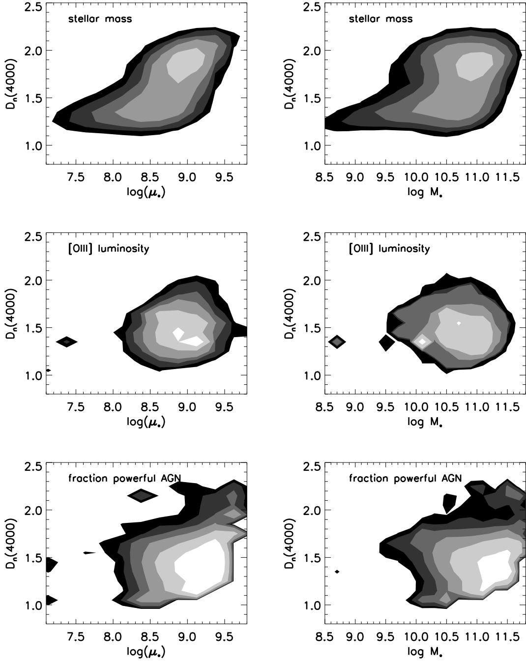
Figure 23: Top: The distribution of the total stellar mass density in the D_n(4000)/\mu_* and D_n(4000)/M_* planes. Middle: The distribution of the total [OIII] luminosity density in AGN in the same planes. Contours indicate a factor two decrease in in density. Bottom: The fraction of galaxies that host powerful ( L[\text{OIII}] > 10^7 L_\odot ) AGN. The contours represent AGN fractions of 0.3, 0.15, 0.07, 0.035, 0.017 and 0.008.
